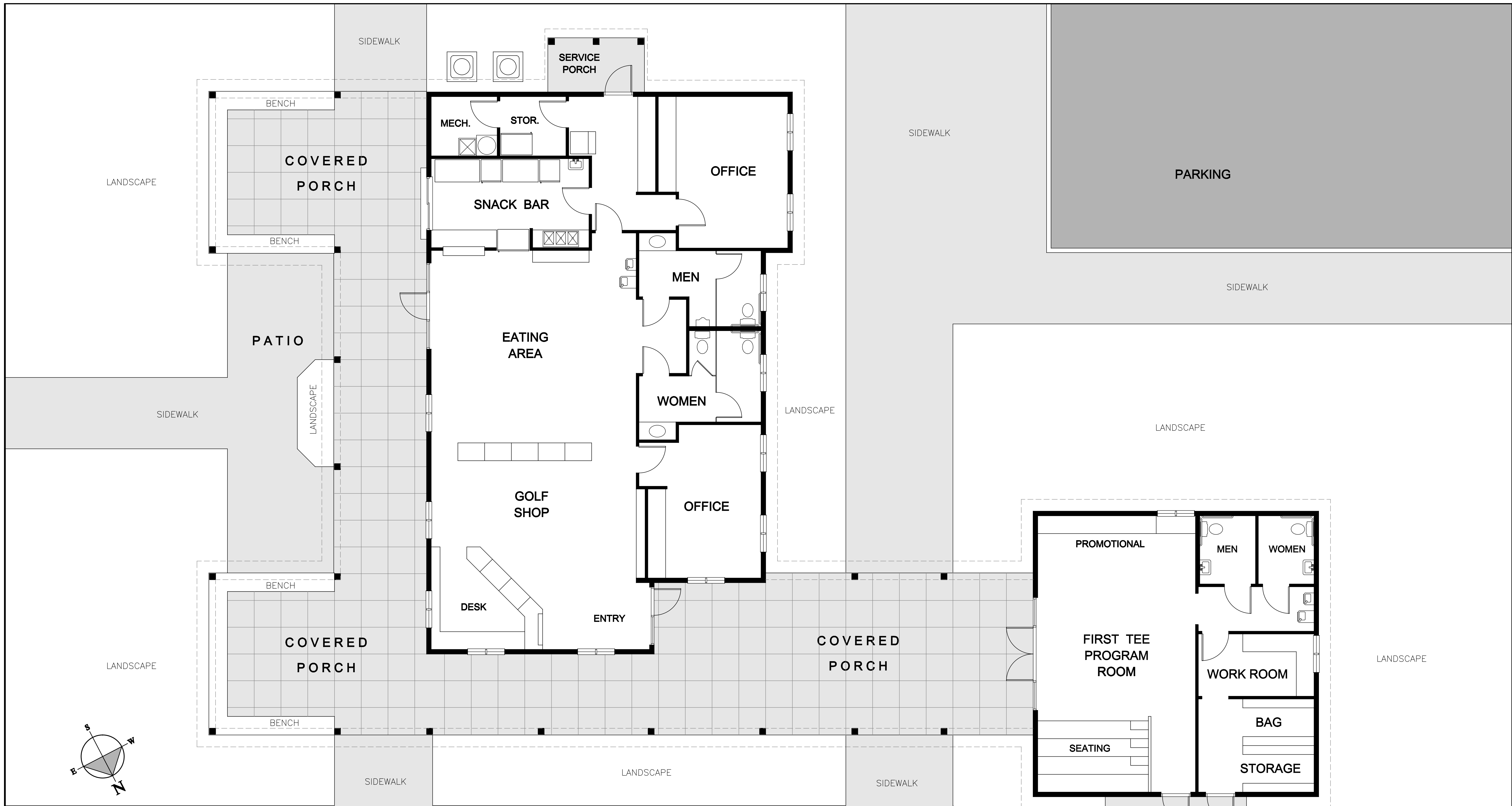
FIRST FLOOR PLAN COVERED PORCHES = 2,412 Sq.Ft. ENCLOSED BUILDINGS = 3,372 Sq.Ft.
