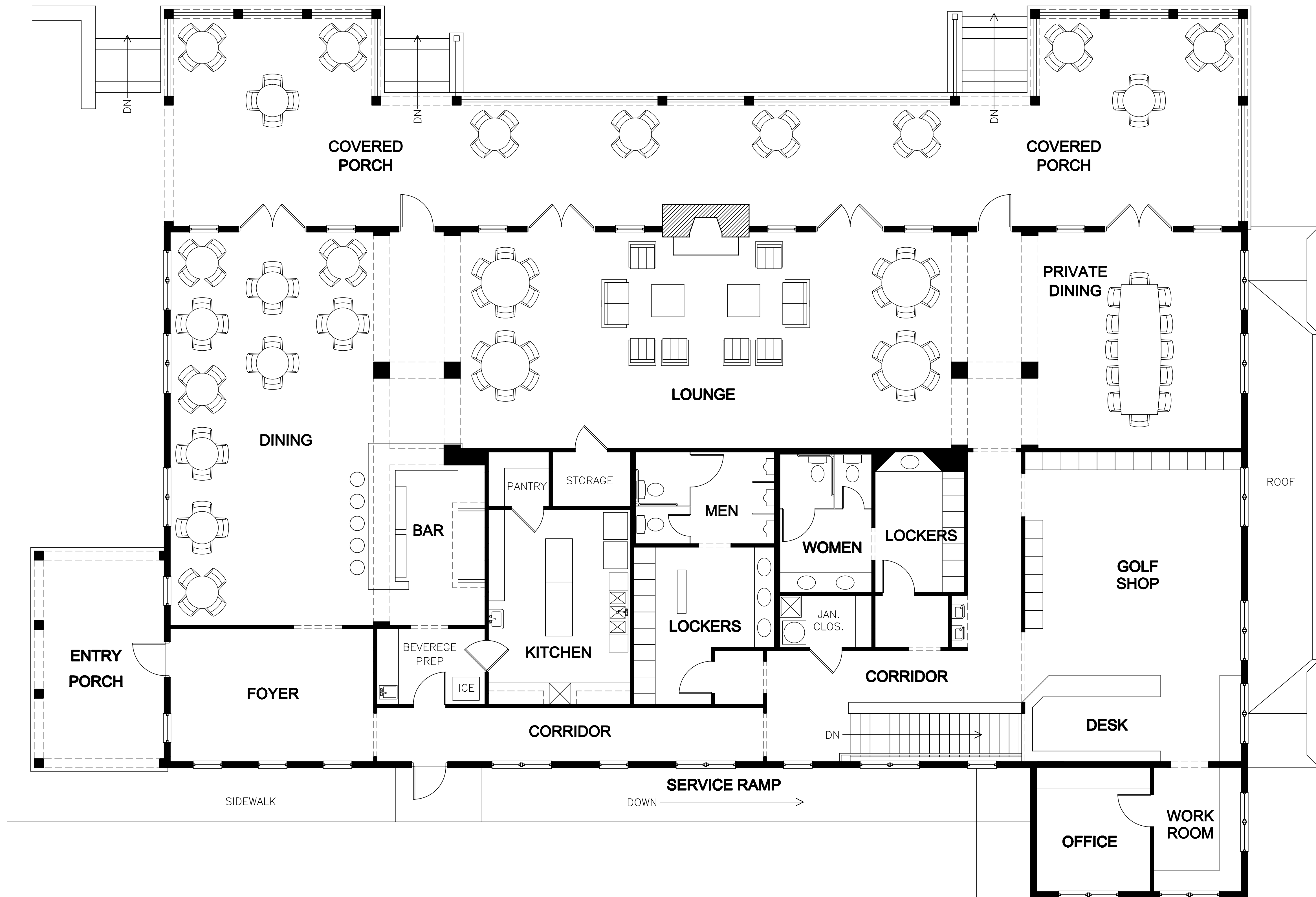
UPPER FLOOR PLAN COVERED PORCHES = 1,760 Sq.Ft. ENCLOSED BUILDING = 5,240 Sq.Ft.
